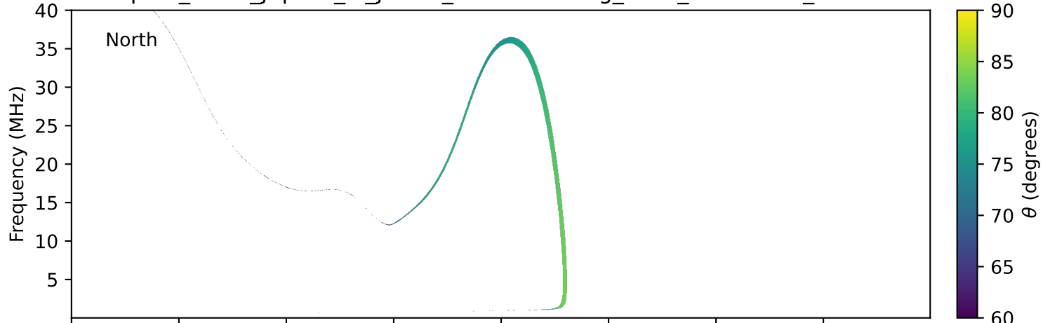
expres_earth_jupiter_io_jrm33_lossc-wid1deg_3kev_20020120_v11.cdf
