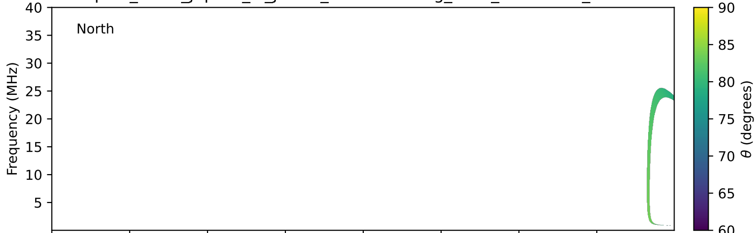
expres_earth_jupiter_io_jrm33_lossc-wid1deg_3kev_20020117_v11.cdf
