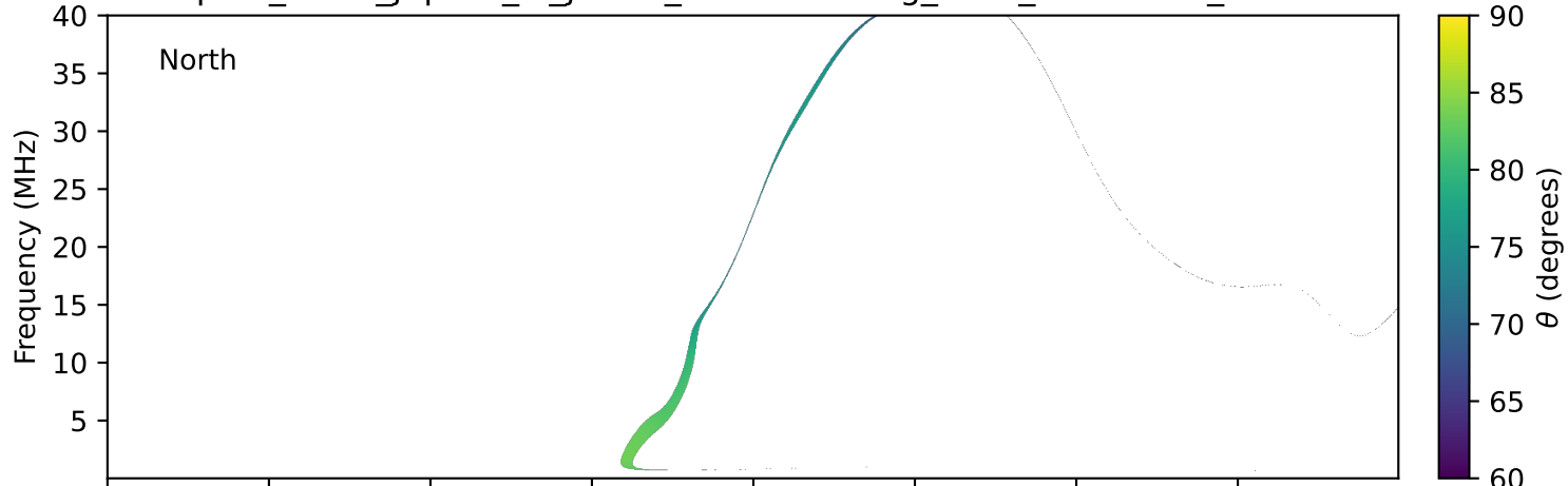
expres_earth_jupiter_io_jrm33_lossc-wid1deg_3kev_20020114_v11.cdf
