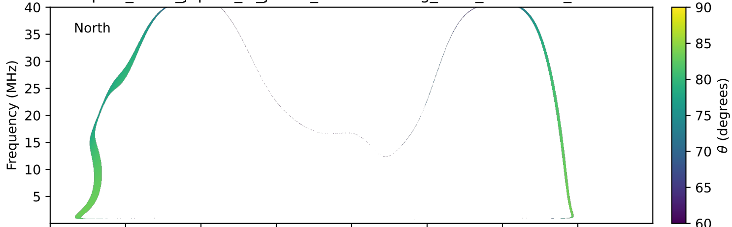
expres_earth_jupiter_io_jrm33_lossc-wid1deg_3kev_20020102_v11.cdf
