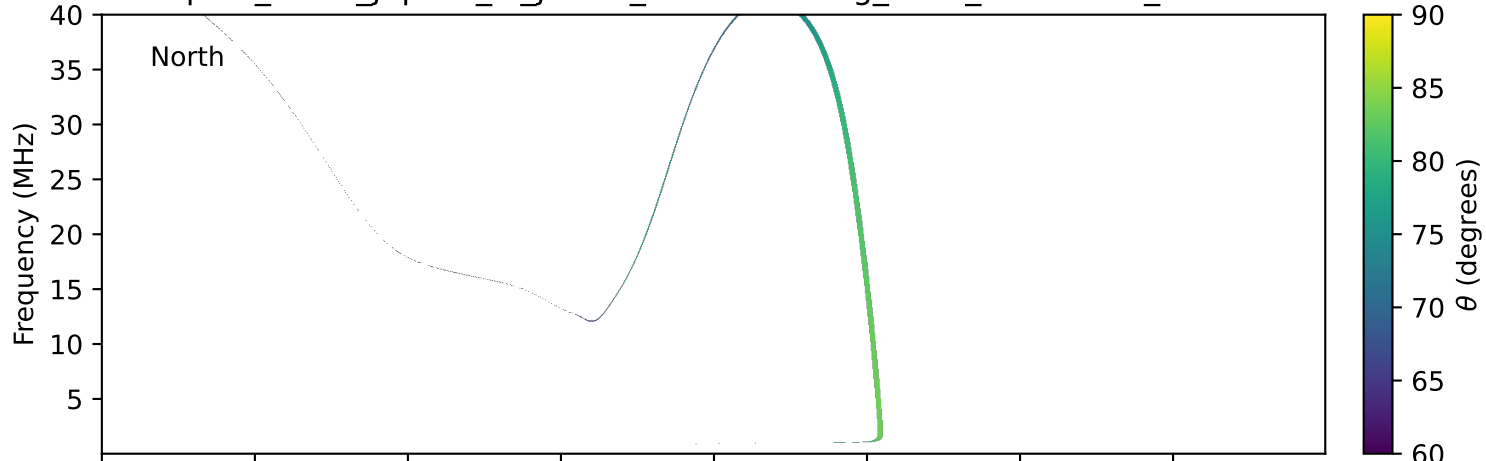
expres_earth_jupiter_io_jrm09_lossc-wid1deg_3kev_20020127_v11.cdf
