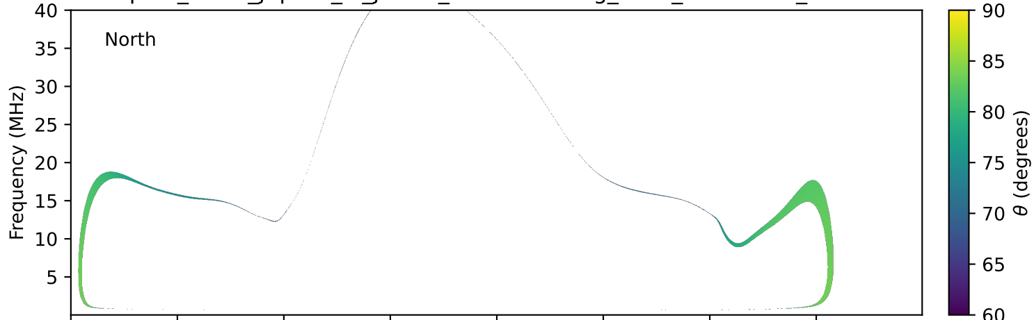
expres_earth_jupiter_io_jrm09_lossc-wid1deg_3kev_20020125_v11.cdf
