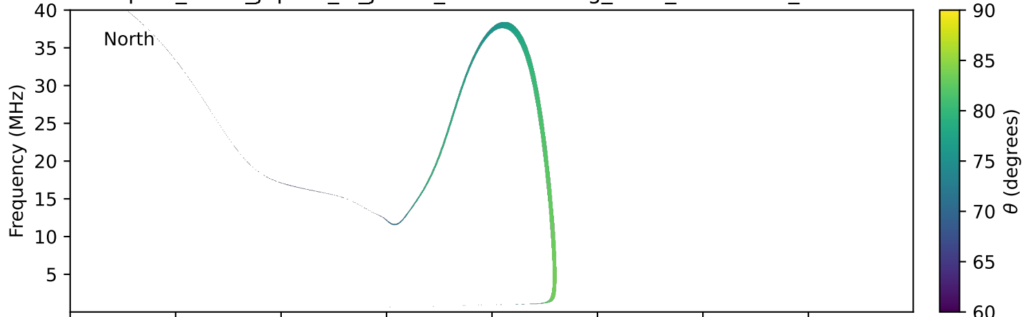
expres_earth_jupiter_io_jrm09_lossc-wid1deg_3kev_20020120_v11.cdf
