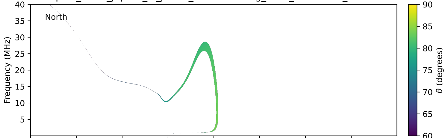
expres_earth_jupiter_io_jrm09_lossc-wid1deg_3kev_20020113_v11.cdf
