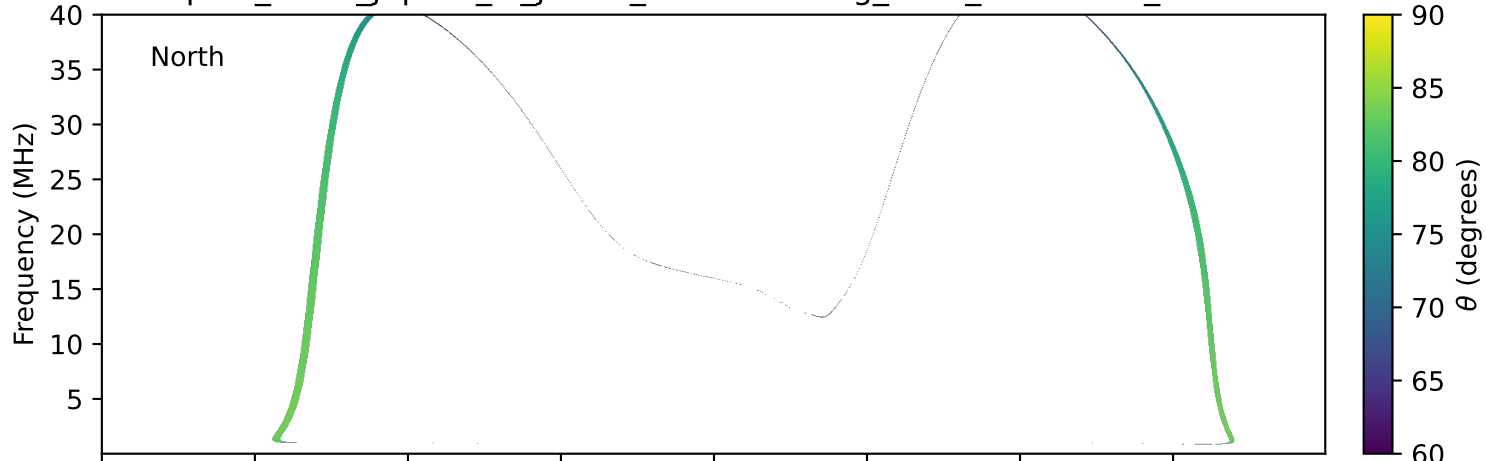
expres_earth_jupiter_io_jrm09_lossc-wid1deg_3kev_20020109_v11.cdf
