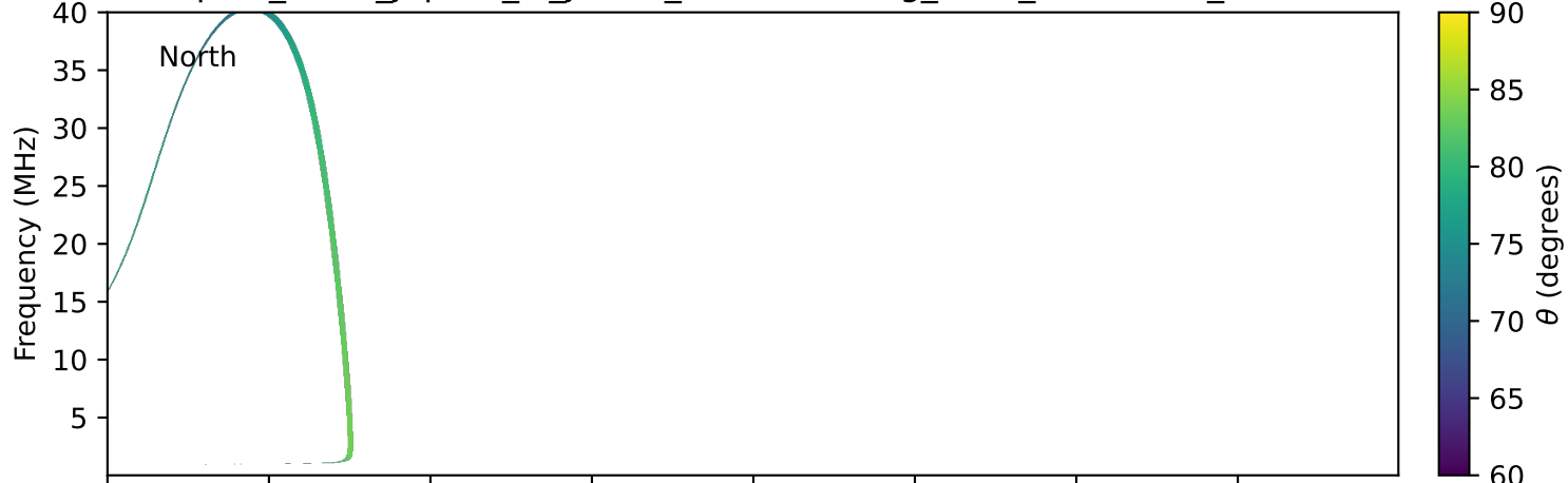
expres_earth_jupiter_io_jrm09_lossc-wid1deg_3kev_20020108_v11.cdf
