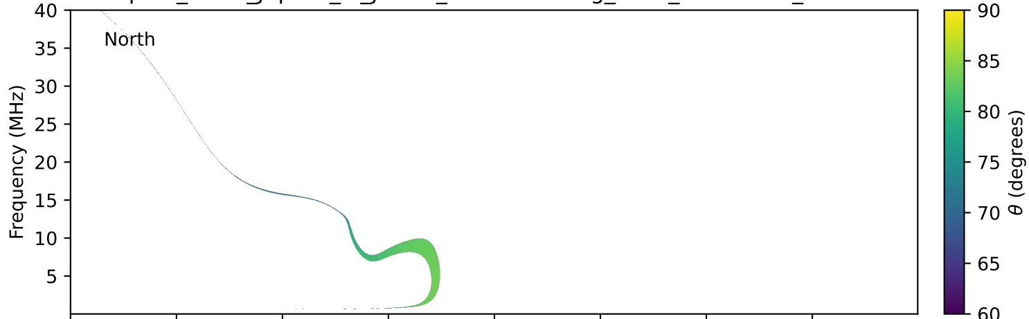
expres_earth_jupiter_io_jrm09_lossc-wid1deg_3kev_20020106_v11.cdf
