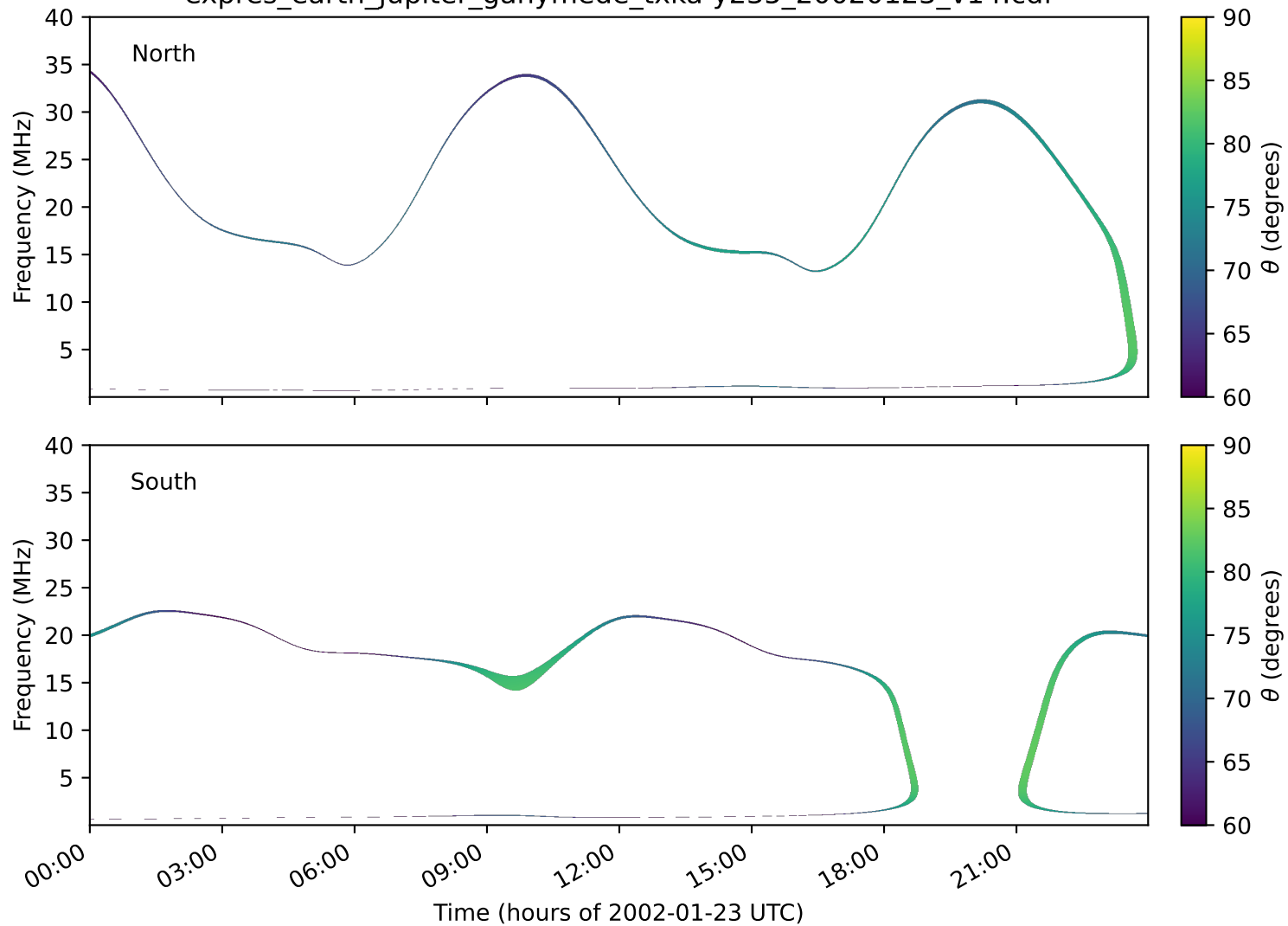
expres_earth_jupiter_ganymede_txka-y235_20020123_v14.cdf
