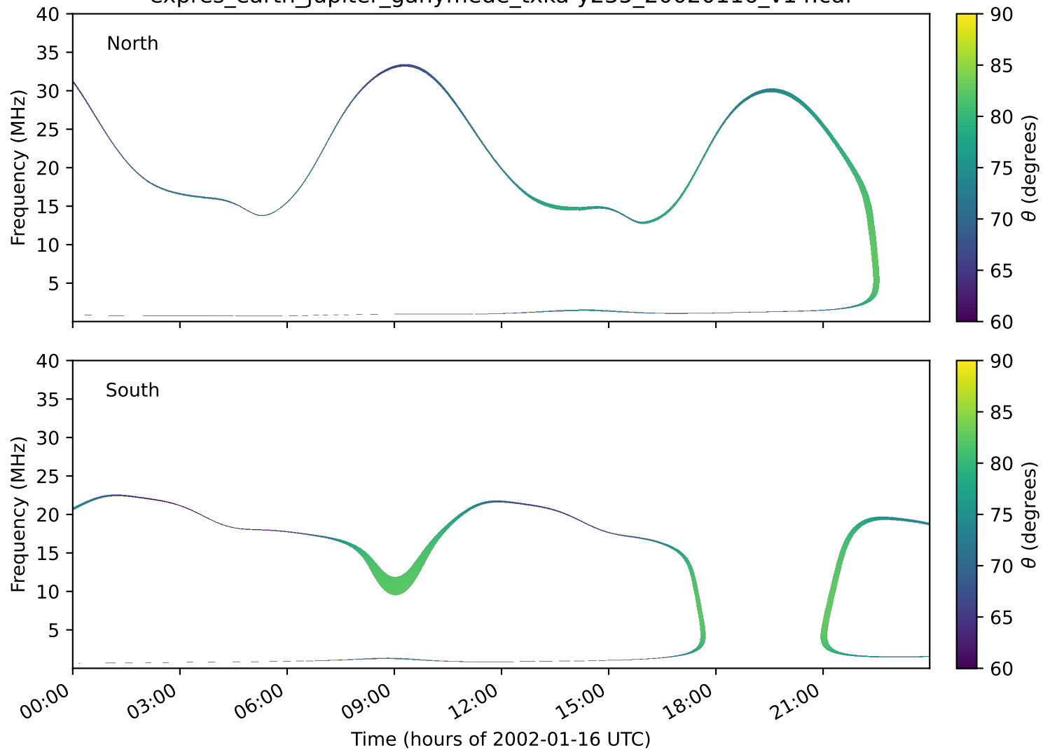
expres_earth_jupiter_ganymede_txka-y235_20020116_v14.cdf
