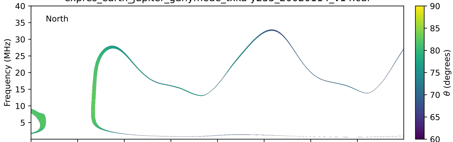
expres_earth_jupiter_ganymede_txka-y235_20020114_v14.cdf
