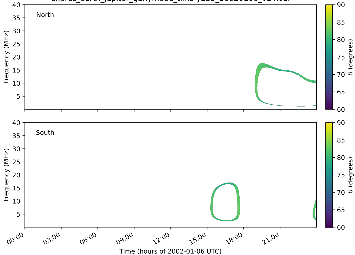
expres_earth_jupiter_ganymede_txka-y235_20020106_v14.cdf
