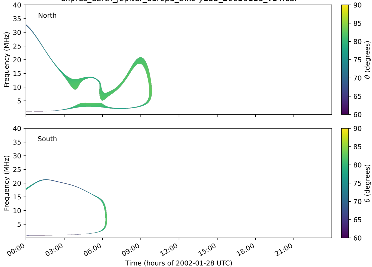
expres_earth_jupiter_europa_txka-y235_20020128_v14.cdf
