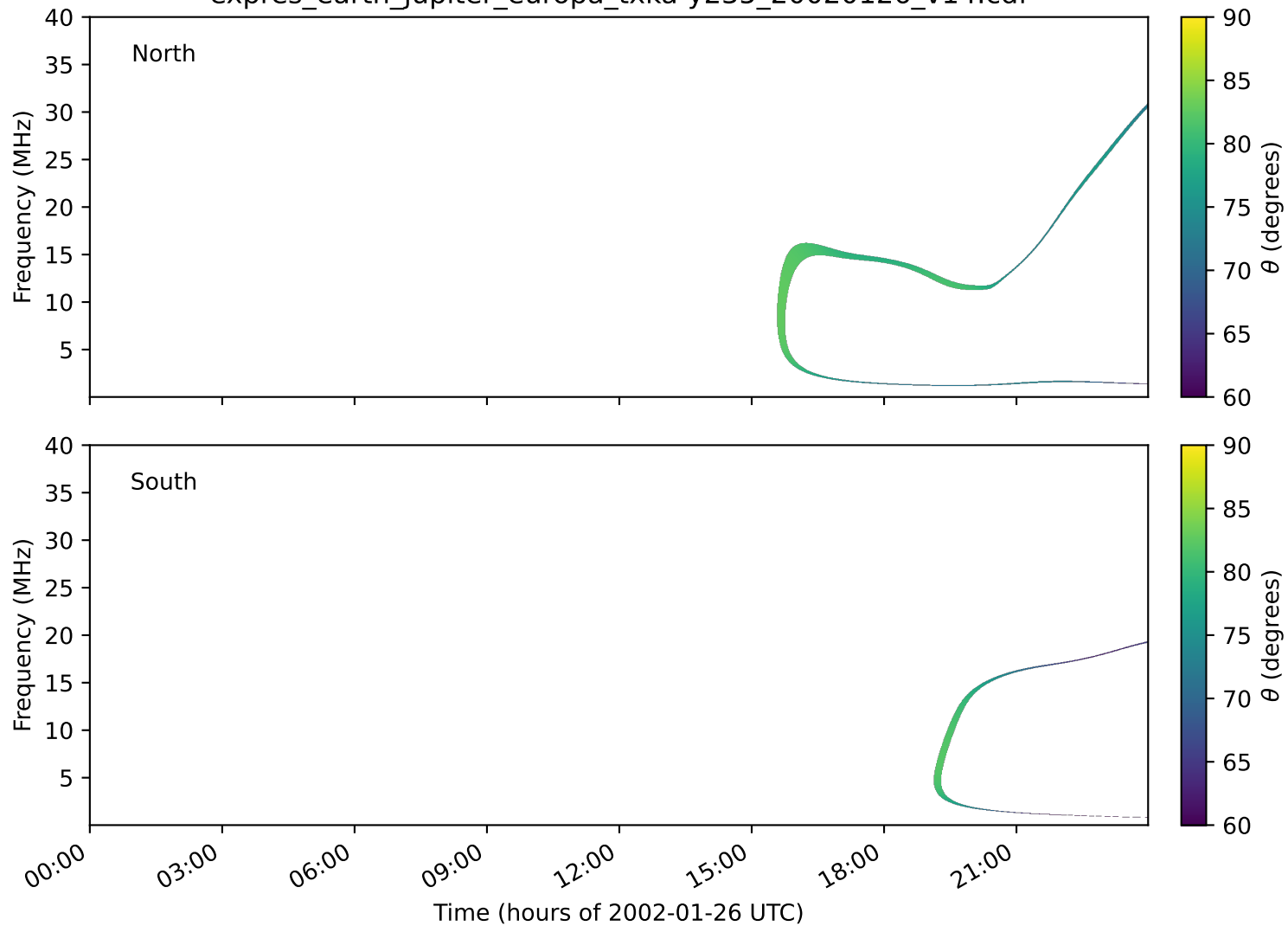
expres_earth_jupiter_europa_txka-y235_20020126_v14.cdf
