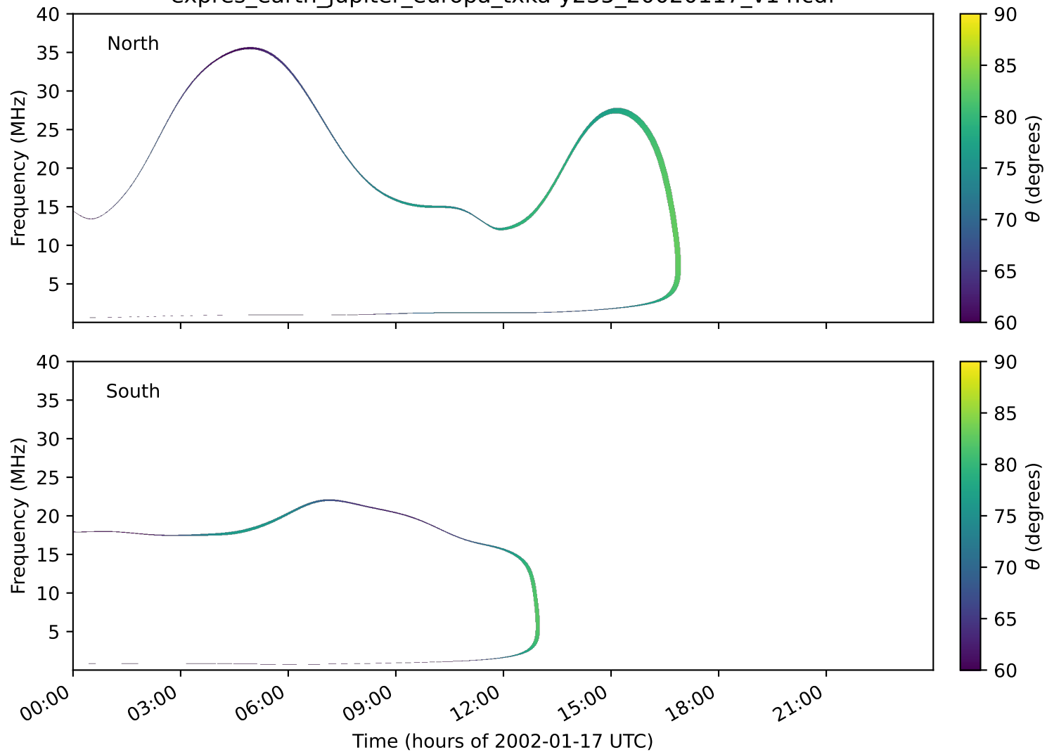
expres_earth_jupiter_europa_txka-y235_20020117_v14.cdf
