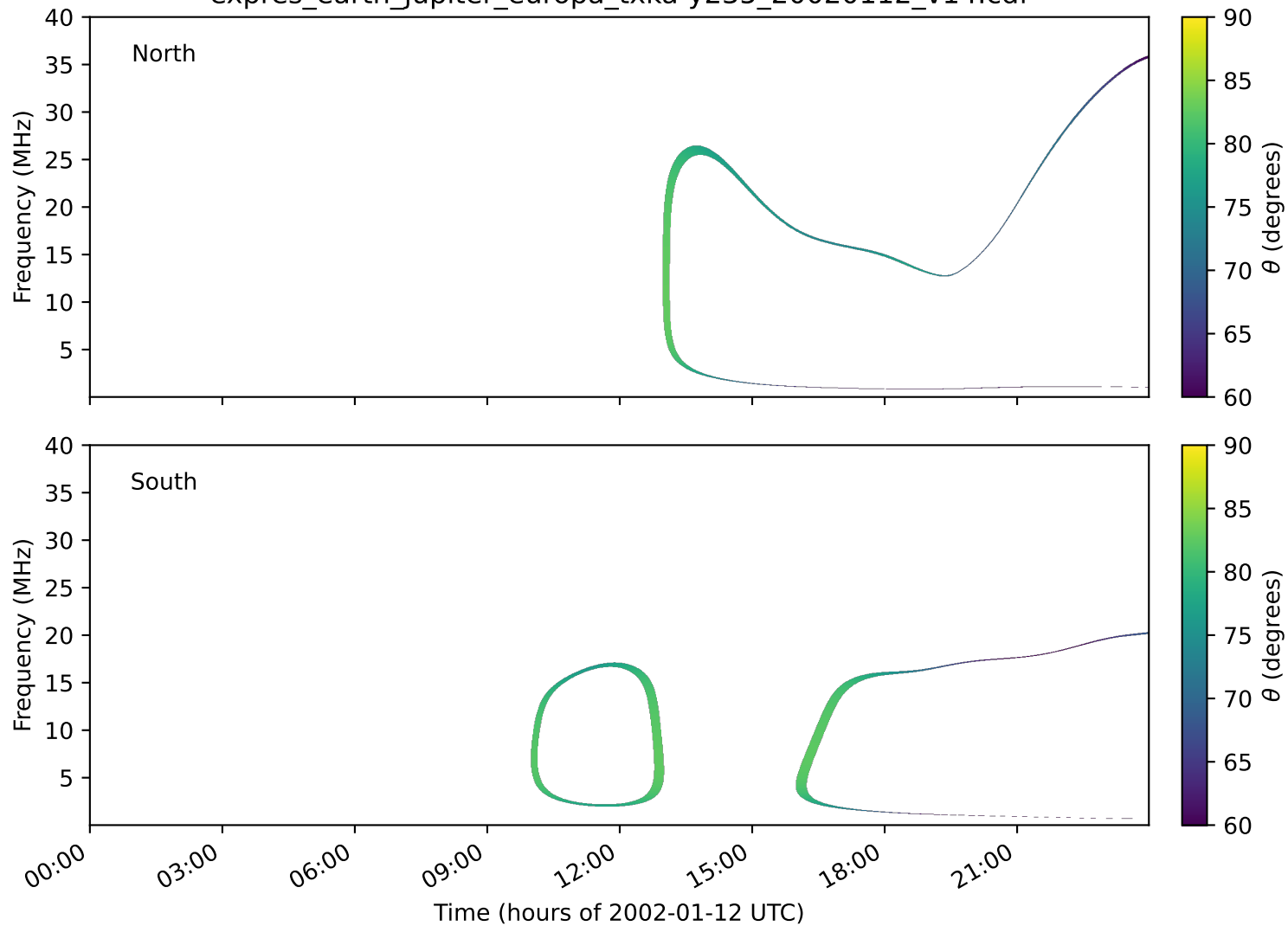
expres_earth_jupiter_europa_txka-y235_20020112_v14.cdf
