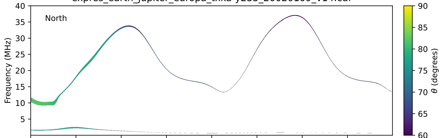
expres_earth_jupiter_europa_txka-y235_20020109_v14.cdf
