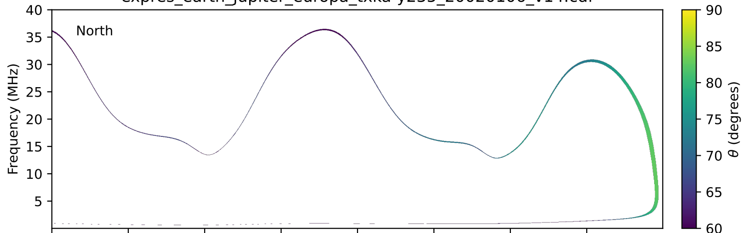
expres_earth_jupiter_europa_txka-y235_20020106_v14.cdf
