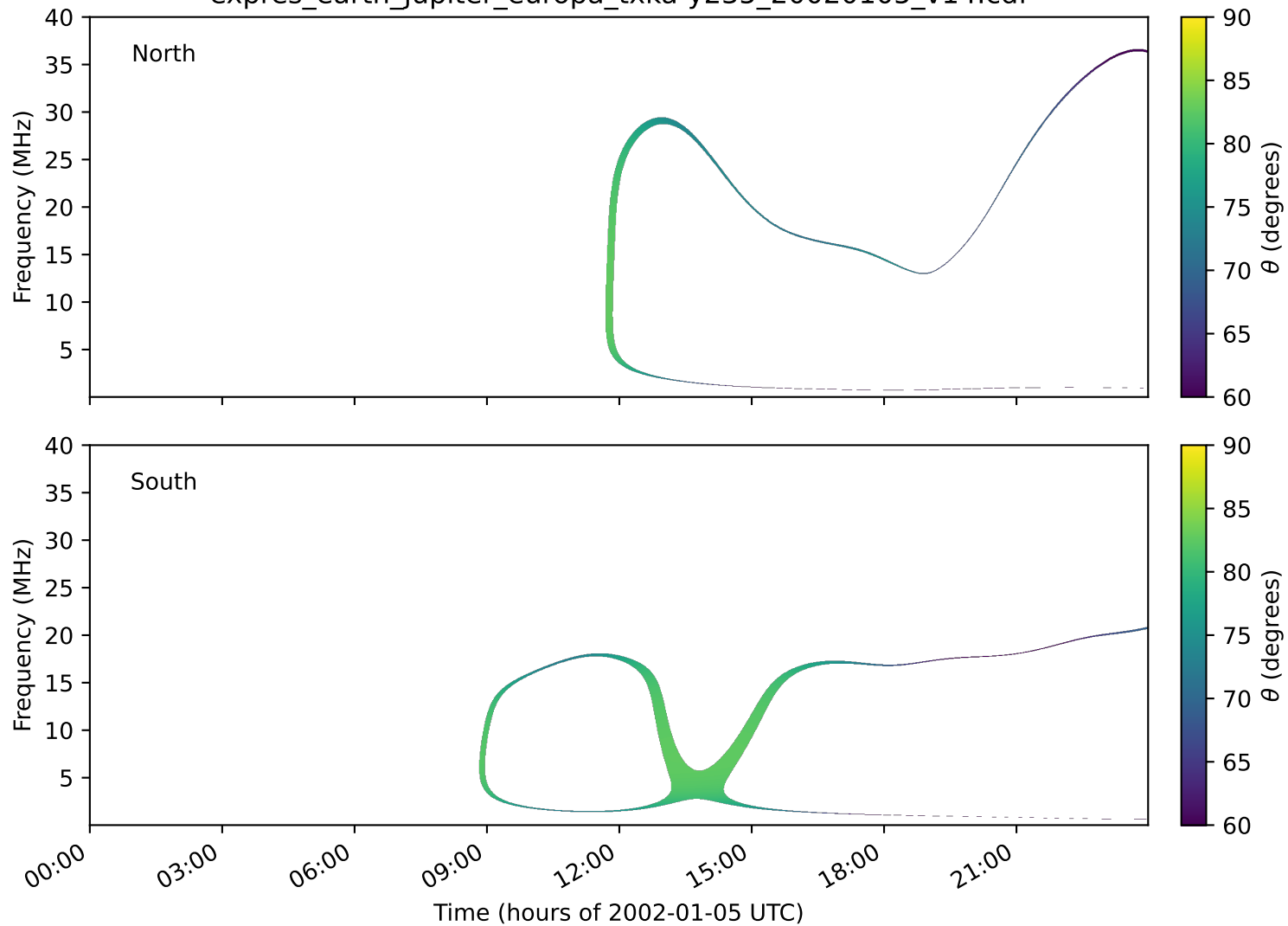
expres_earth_jupiter_europa_txka-y235_20020105_v14.cdf
