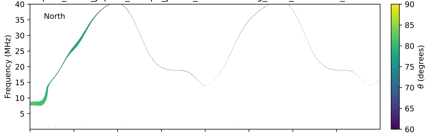
expres_earth_jupiter_europa_jrm33_lossc-wid1deg_3kev_20020102_v11.cdf
