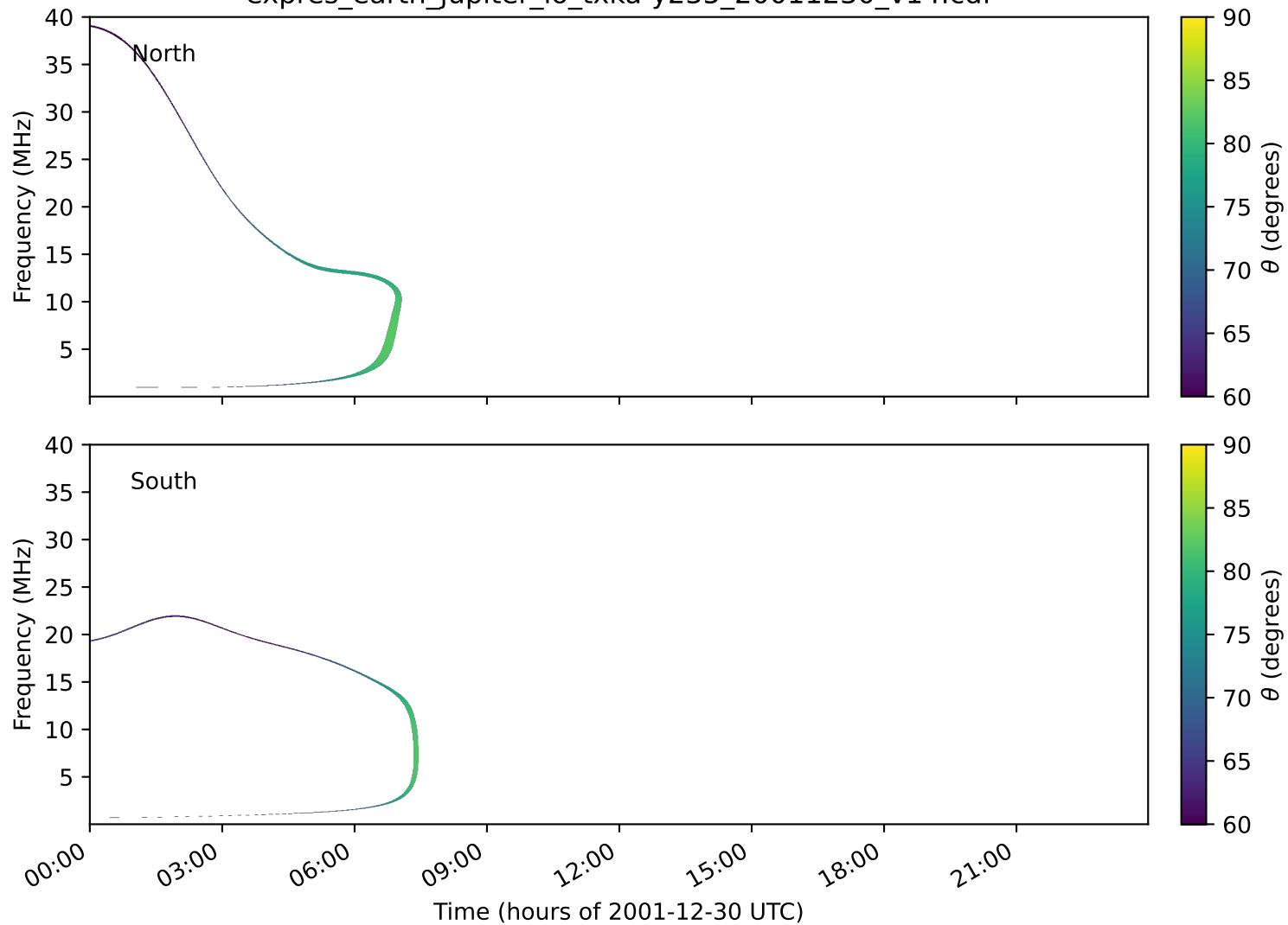
expres_earth_jupiter_io_txka-y235_20011230_v14.cdf
