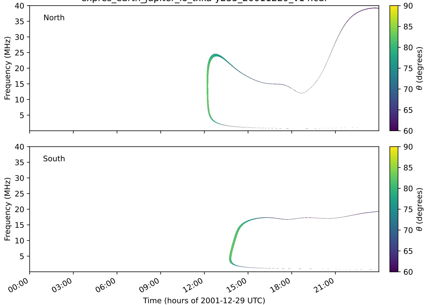
expres_earth_jupiter_io_txka-y235_20011229_v14.cdf
