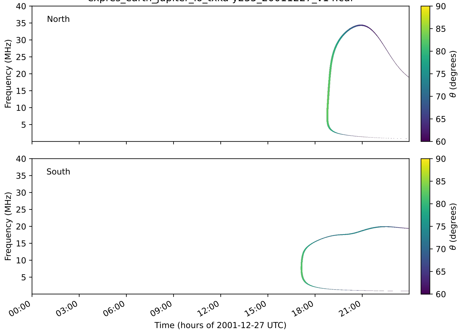
expres_earth_jupiter_io_txka-y235_20011227_v14.cdf
