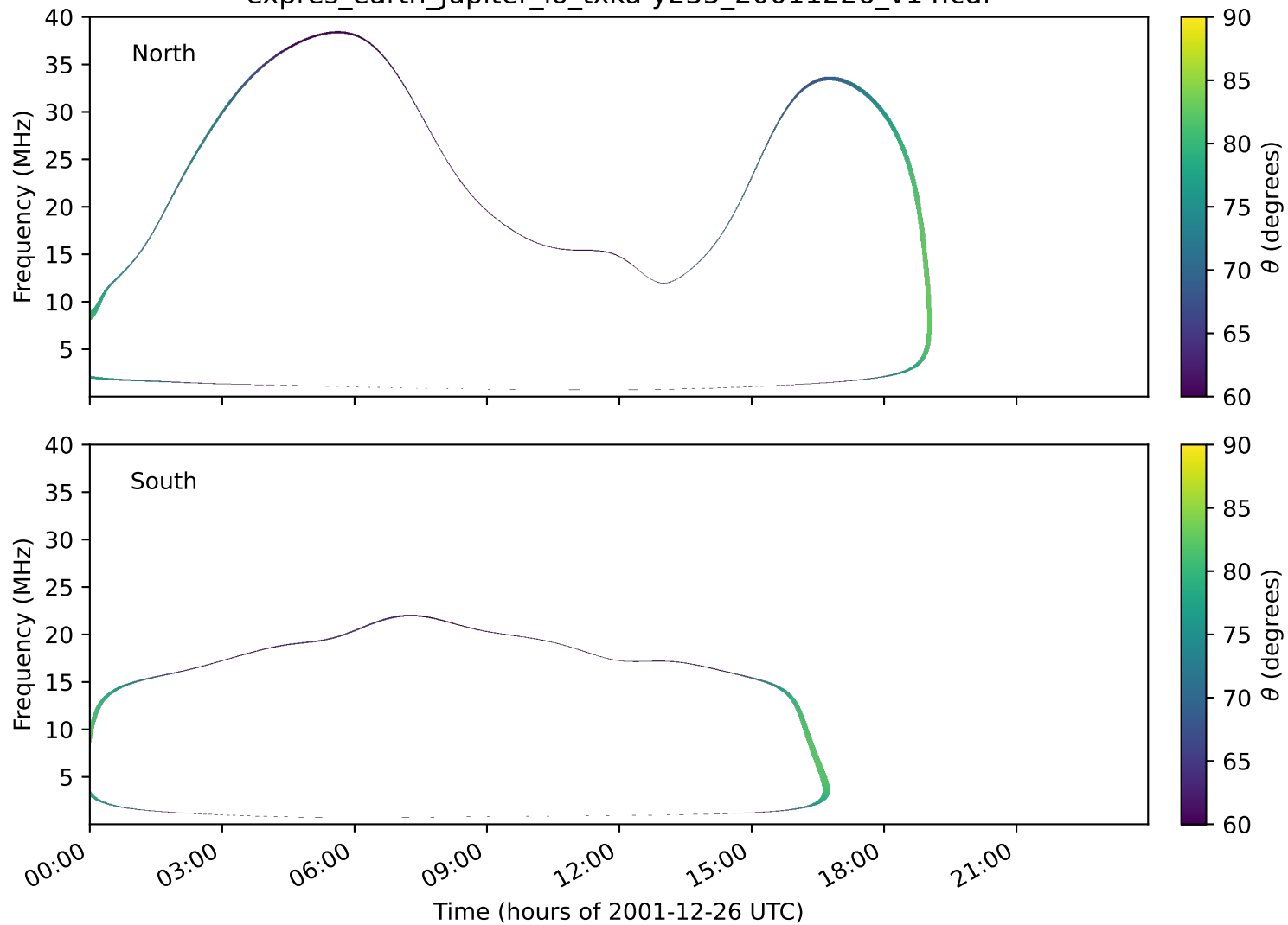
expres_earth_jupiter_io_txka-y235_20011226_v14.cdf
