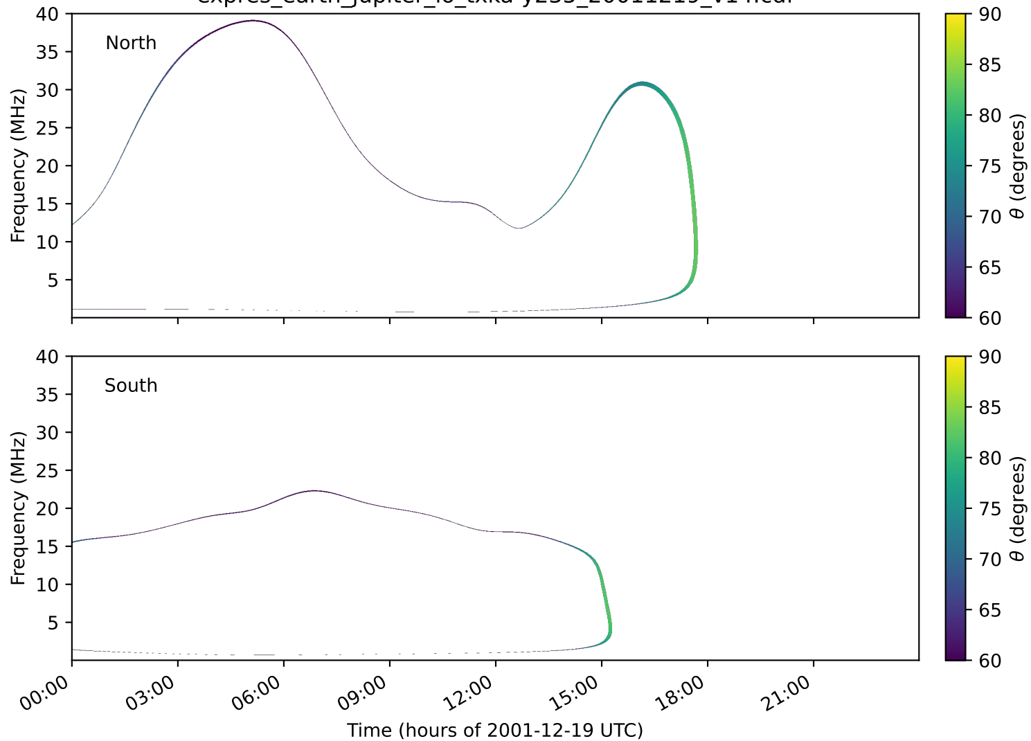
expres_earth_jupiter_io_txka-y235_20011219_v14.cdf
