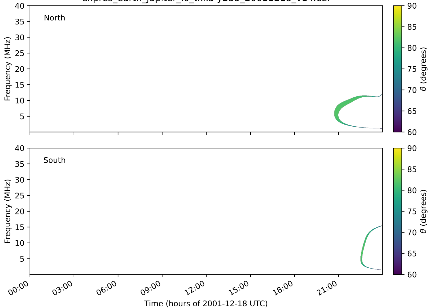
expres_earth_jupiter_io_txka-y235_20011218_v14.cdf
