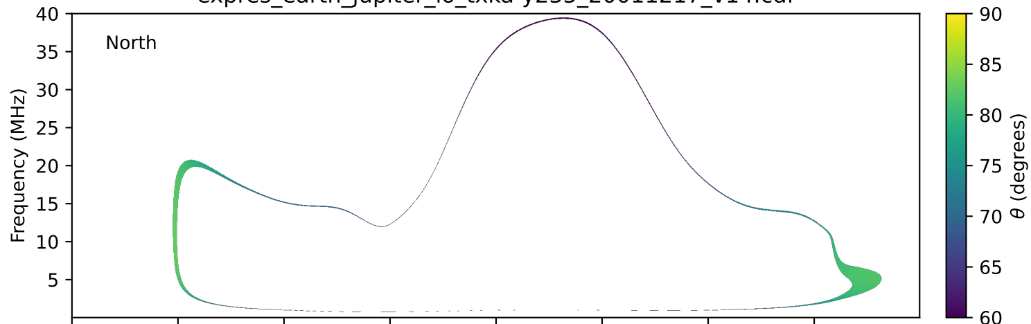
expres_earth_jupiter_io_txka-y235_20011217_v14.cdf
