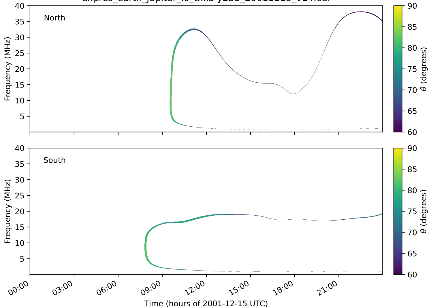
expres_earth_jupiter_io_txka-y235_20011215_v14.cdf
