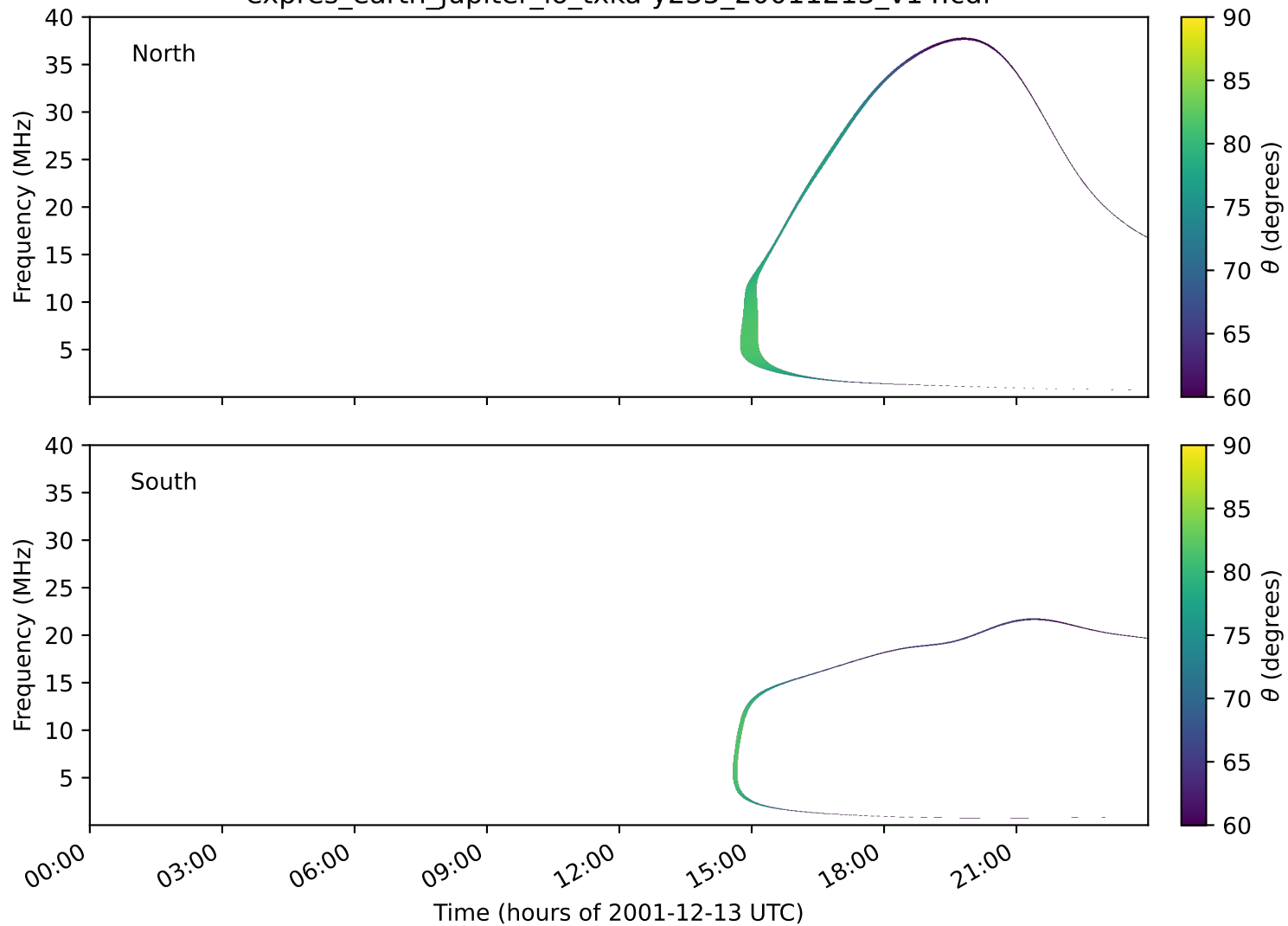
expres_earth_jupiter_io_txka-y235_20011213_v14.cdf
