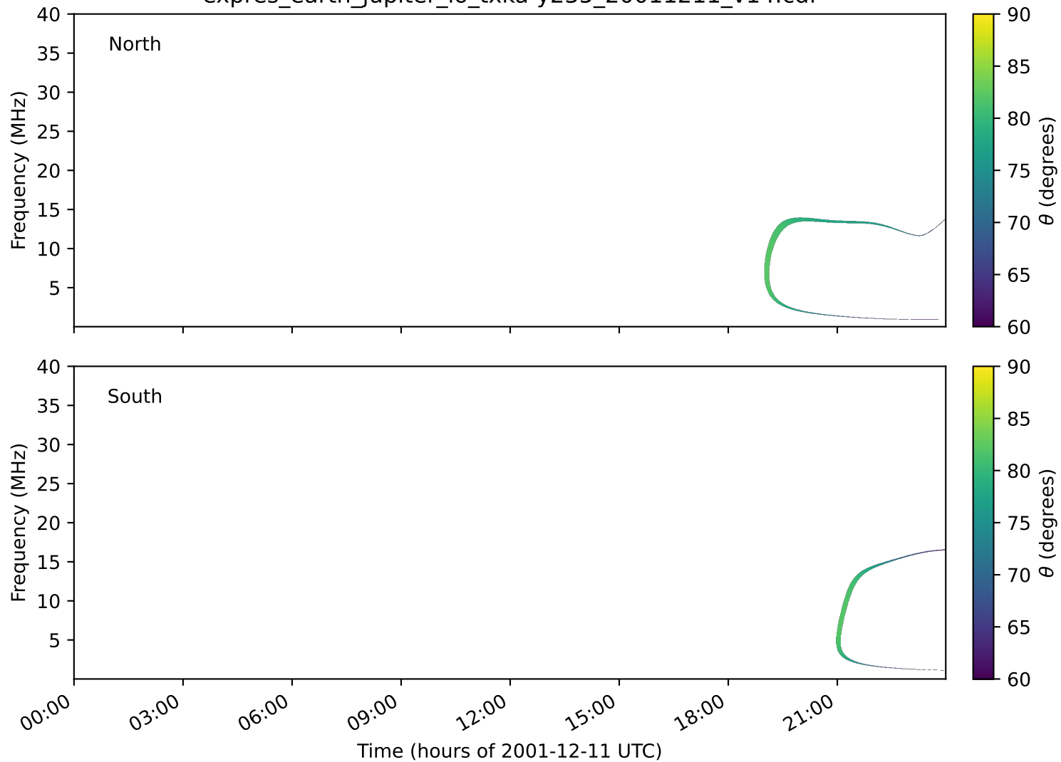
expres_earth_jupiter_io_txka-y235_20011211_v14.cdf
