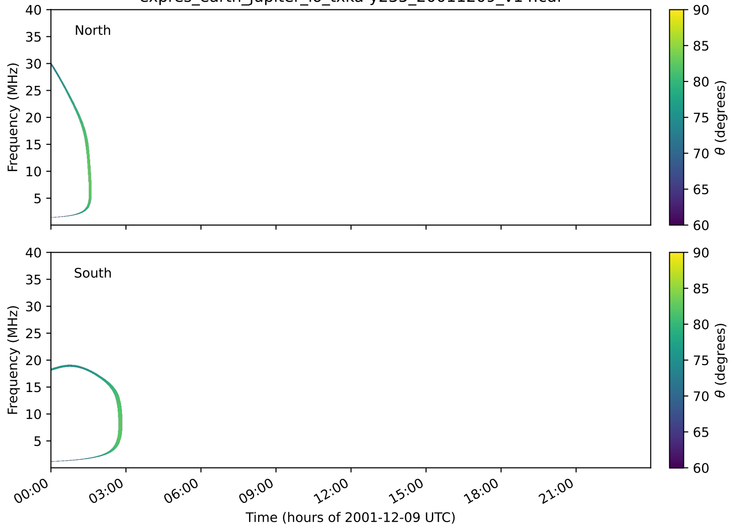
expres_earth_jupiter_io_txka-y235_20011209_v14.cdf
