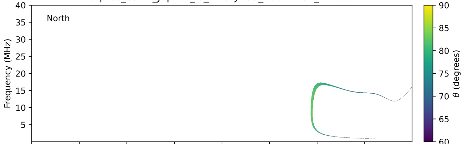
expres_earth_jupiter_io_txka-y235_20011204_v14.cdf
