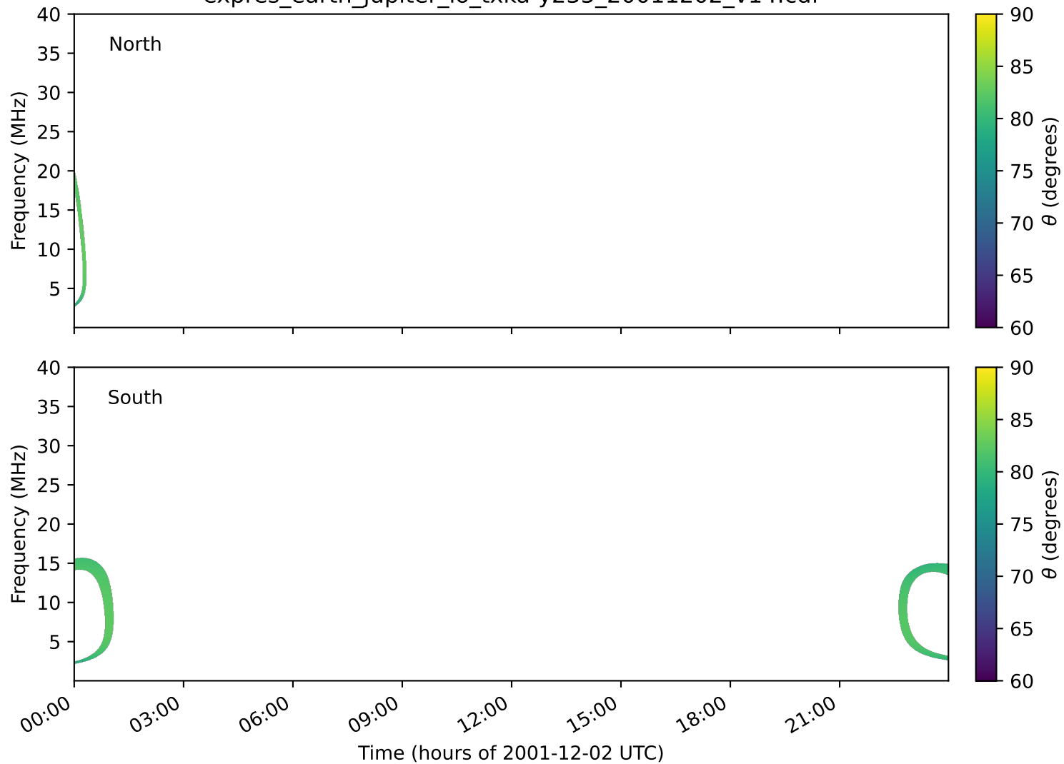
expres_earth_jupiter_io_txka-y235_20011202_v14.cdf
