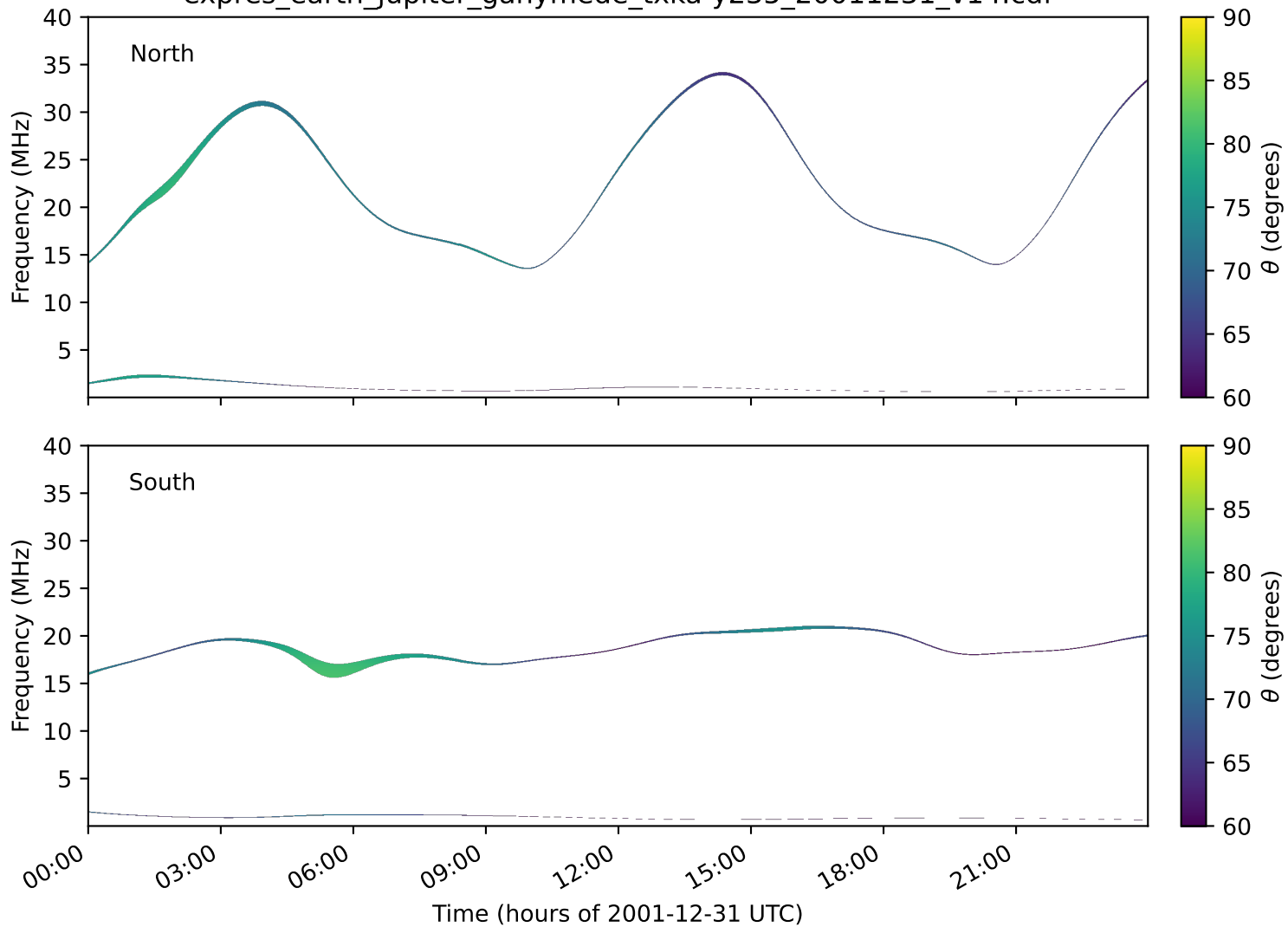
expres_earth_jupiter_ganymede_txka-y235_20011231_v14.cdf
