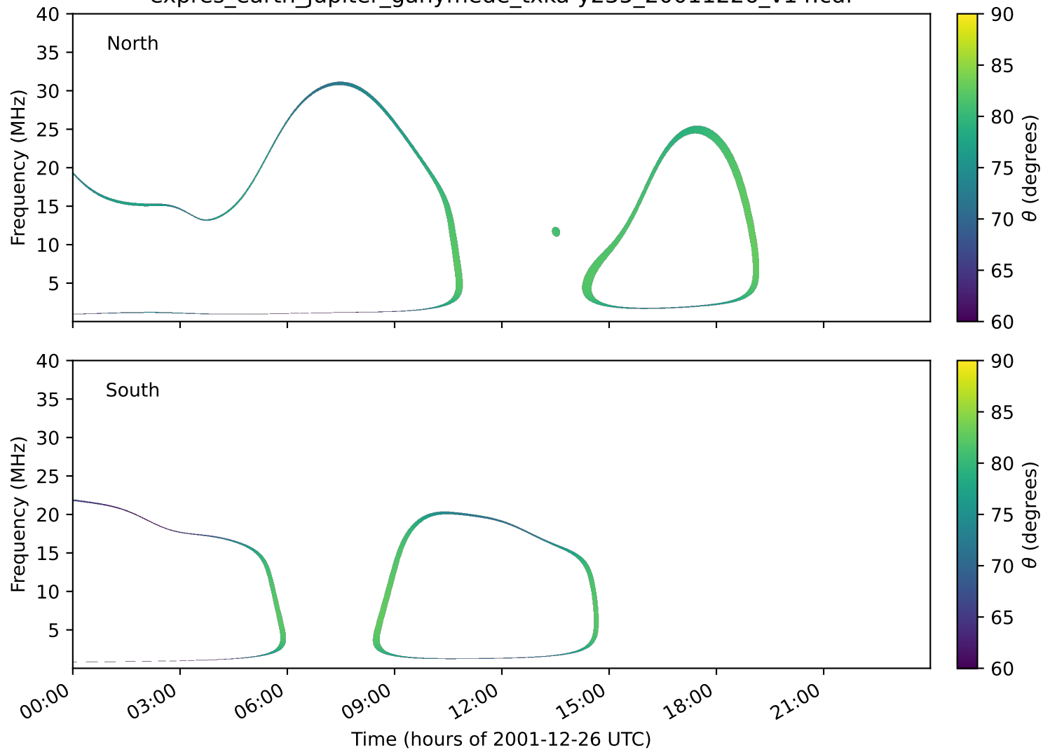
expres_earth_jupiter_ganymede_txka-y235_20011226_v14.cdf
