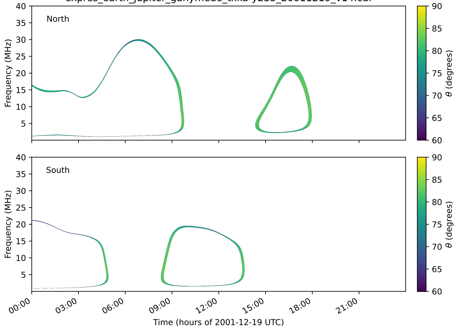
expres_earth_jupiter_ganymede_txka-y235_20011219_v14.cdf
