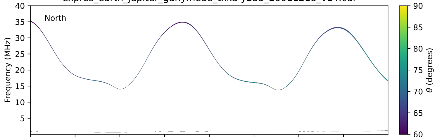
expres_earth_jupiter_ganymede_txka-y235_20011218_v14.cdf
