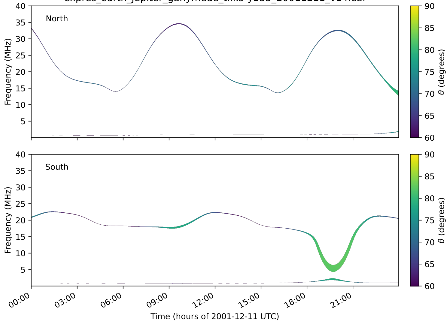
expres_earth_jupiter_ganymede_txka-y235_20011211_v14.cdf
