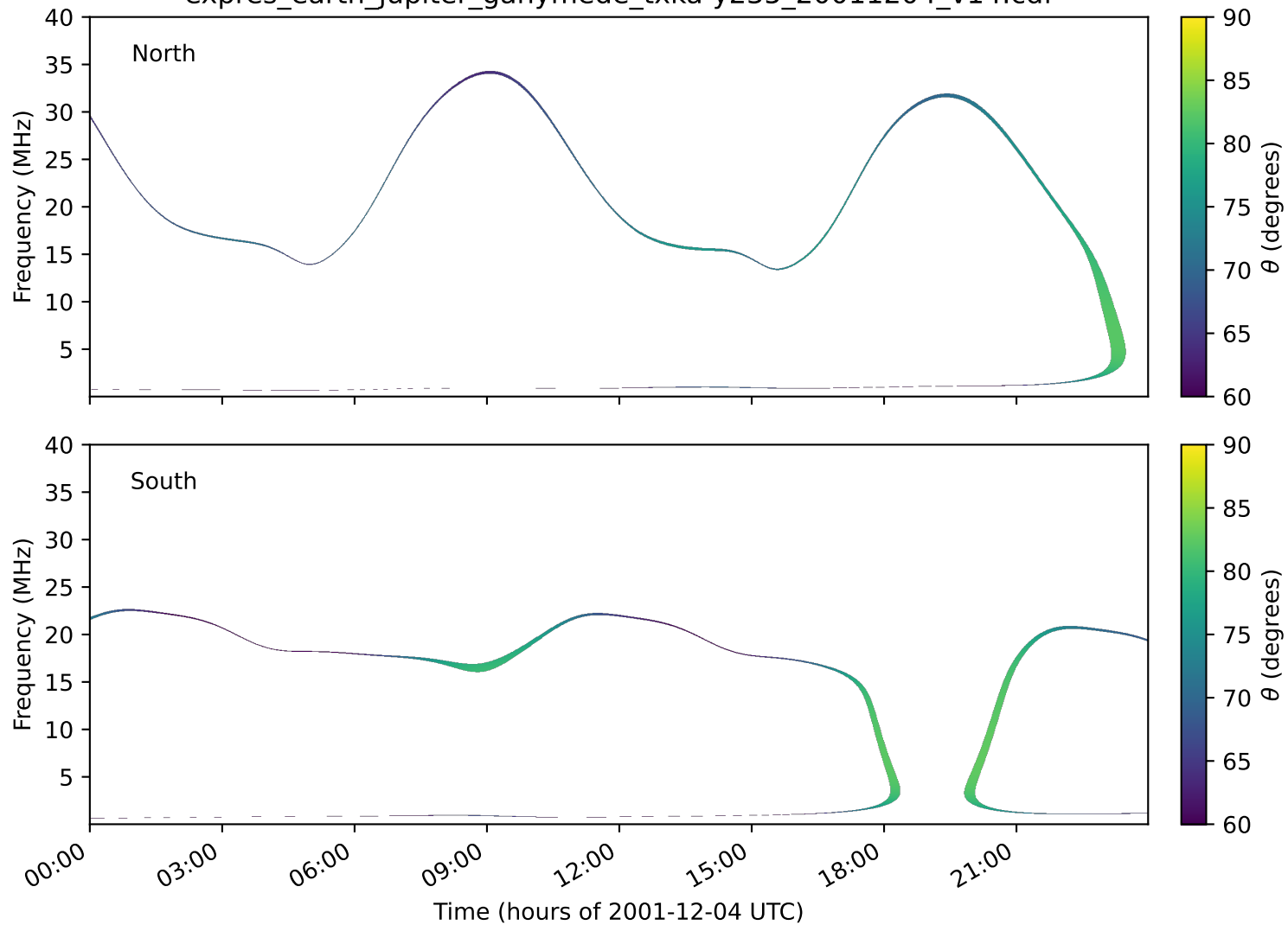
expres_earth_jupiter_ganymede_txka-y235_20011204_v14.cdf
