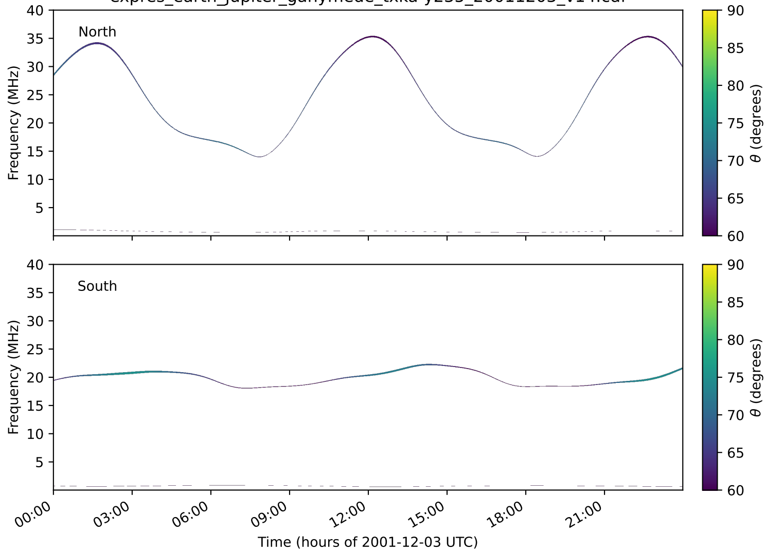
expres_earth_jupiter_ganymede_txka-y235_20011203_v14.cdf
