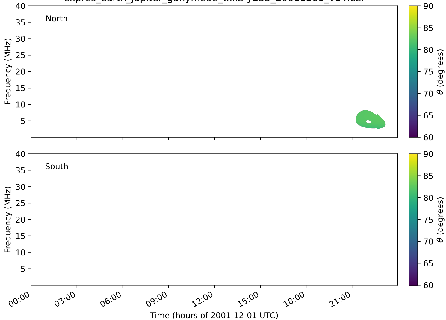
expres_earth_jupiter_ganymede_txka-y235_20011201_v14.cdf
