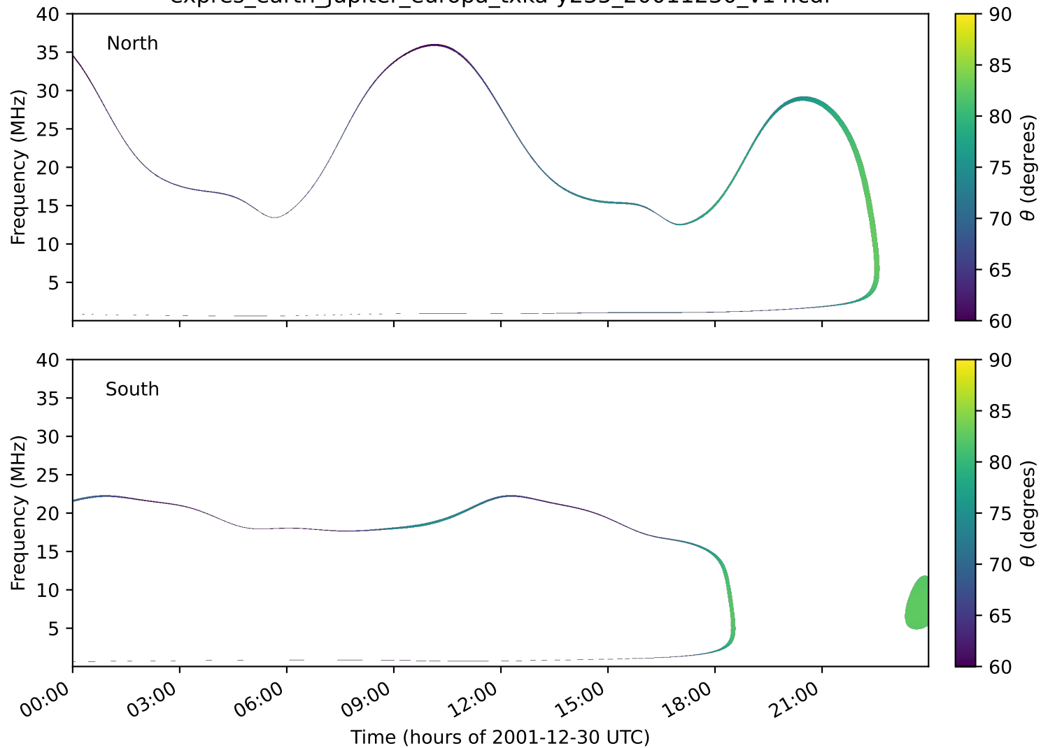
expres_earth_jupiter_europa_txka-y235_20011230_v14.cdf
