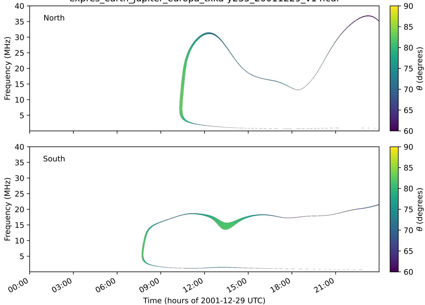
expres_earth_jupiter_europa_txka-y235_20011229_v14.cdf
