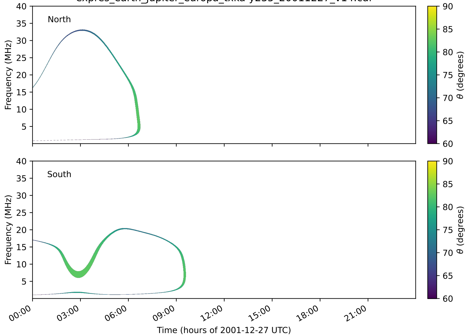
expres_earth_jupiter_europa_txka-y235_20011227_v14.cdf
