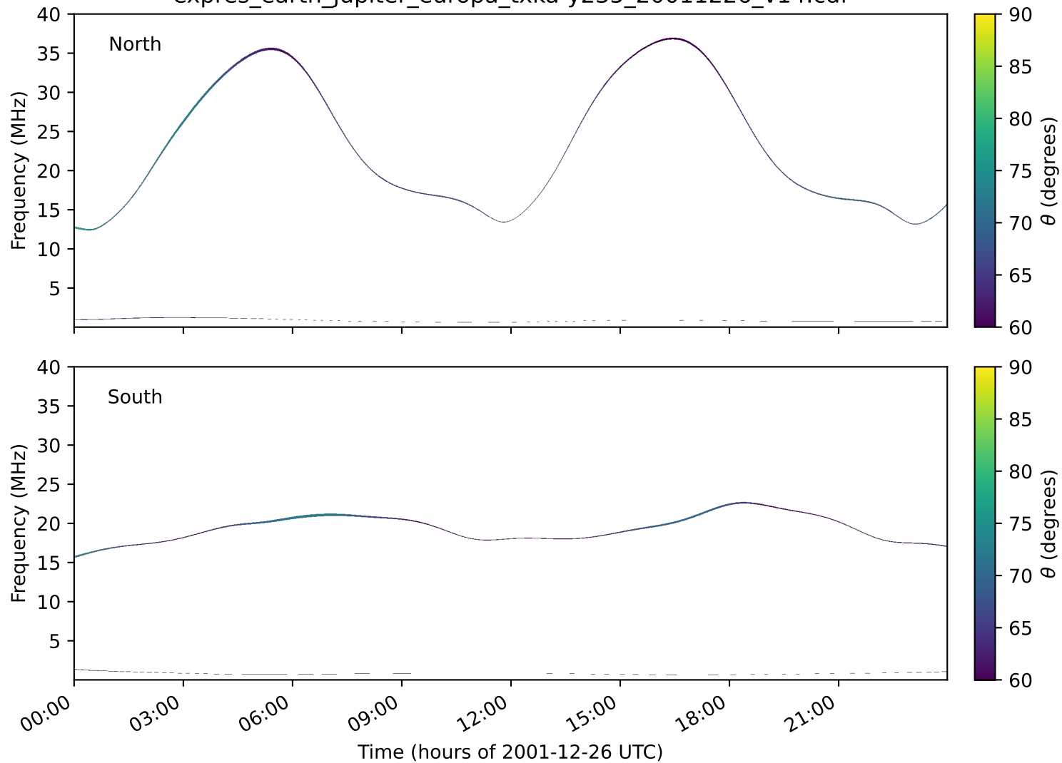
expres_earth_jupiter_europa_txka-y235_20011226_v14.cdf
