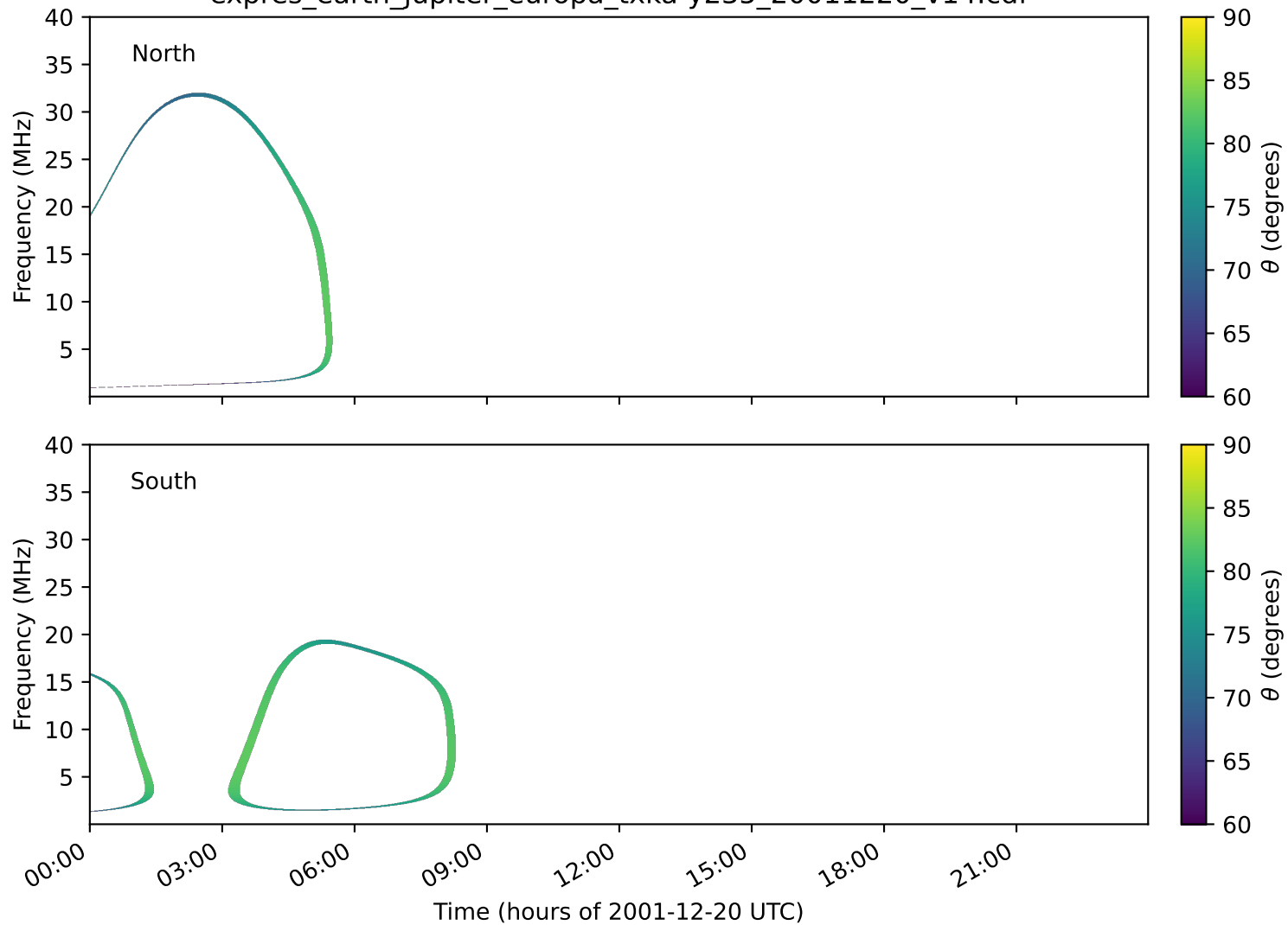
expres_earth_jupiter_europa_txka-y235_20011220_v14.cdf
