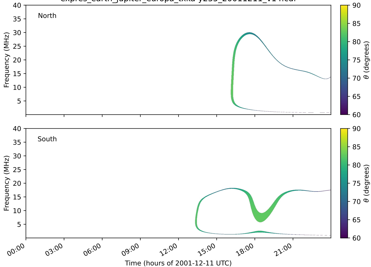
expres_earth_jupiter_europa_txka-y235_20011211_v14.cdf
